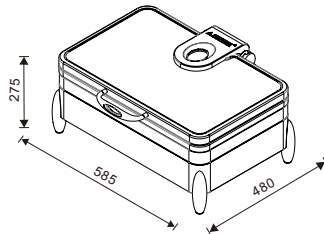
W07-1102T + W07-1104B
