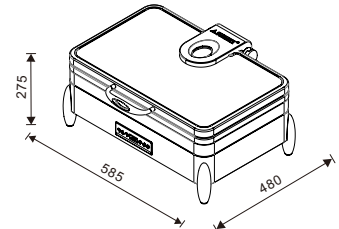
W07-1102T + W07-1102B
