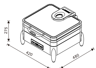
W07-2302T + W07-2302B
